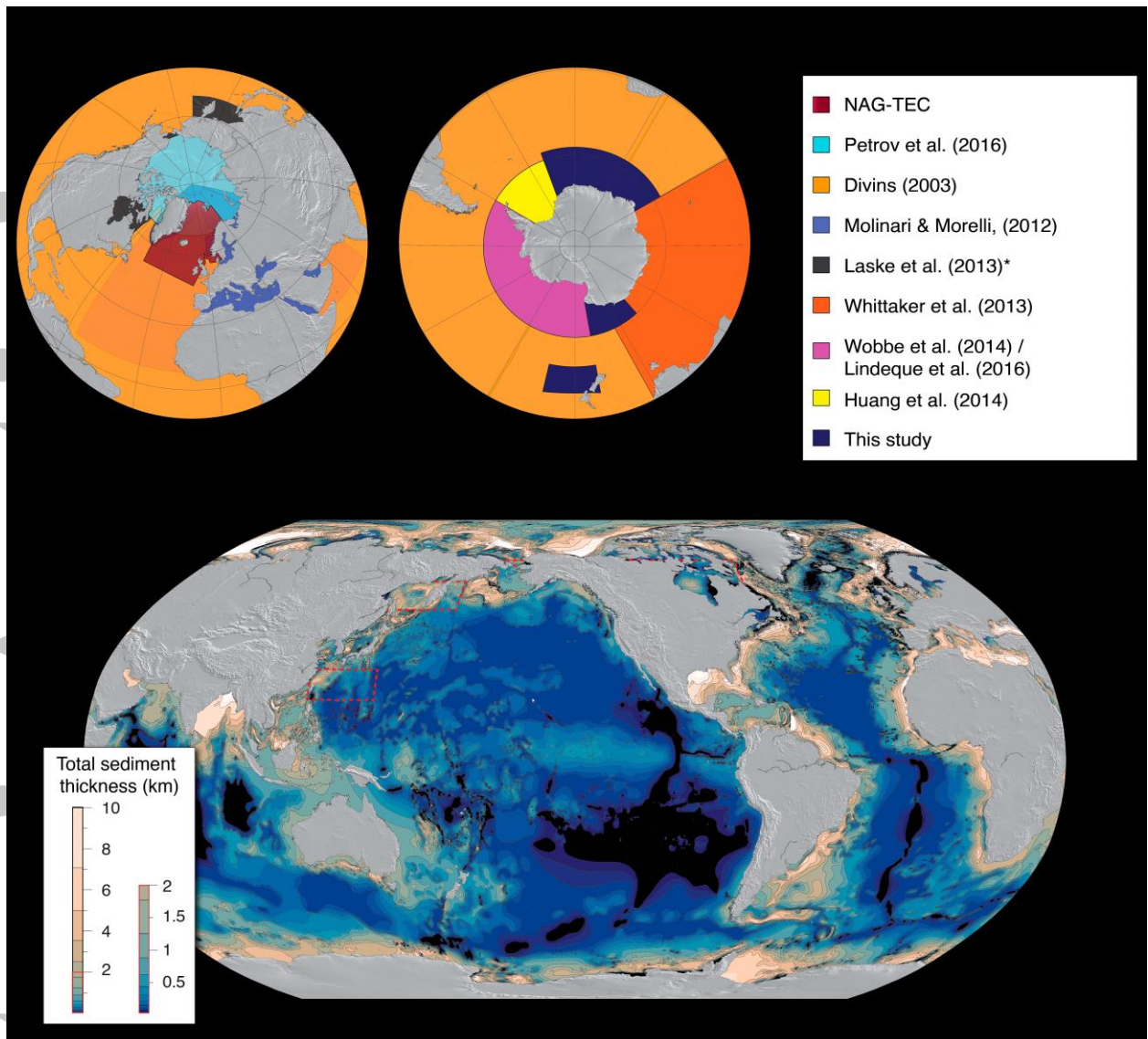
Figure 2: New global total sediment thickness grid, GlobSed. a) Sources of the grids compiled to fill the previously poorly mapped Arctic and the NE Atlantic oceans and the Mediterranean Sea. Darker orange in the Northern Hemisphere indicates the full extent of the Molinari and Morelli (2012) grid, but it was only used in areas colored dark blue (e.g. in the Mediterranean Ocean). b) Sources of the updated sediment thickness map of the Southern Ocean. See color legend and text for references. c) Map showing total sediment thickness in kilometers. Regions inside red dashed polygons indicate sediment thickness values taken from the Laske et al. (2013) grid with an original coarser grid node spacing (1 degree) than the other used grids. This grid was given a lower priority in the grid merging order and is marked (*) in the color legend.
