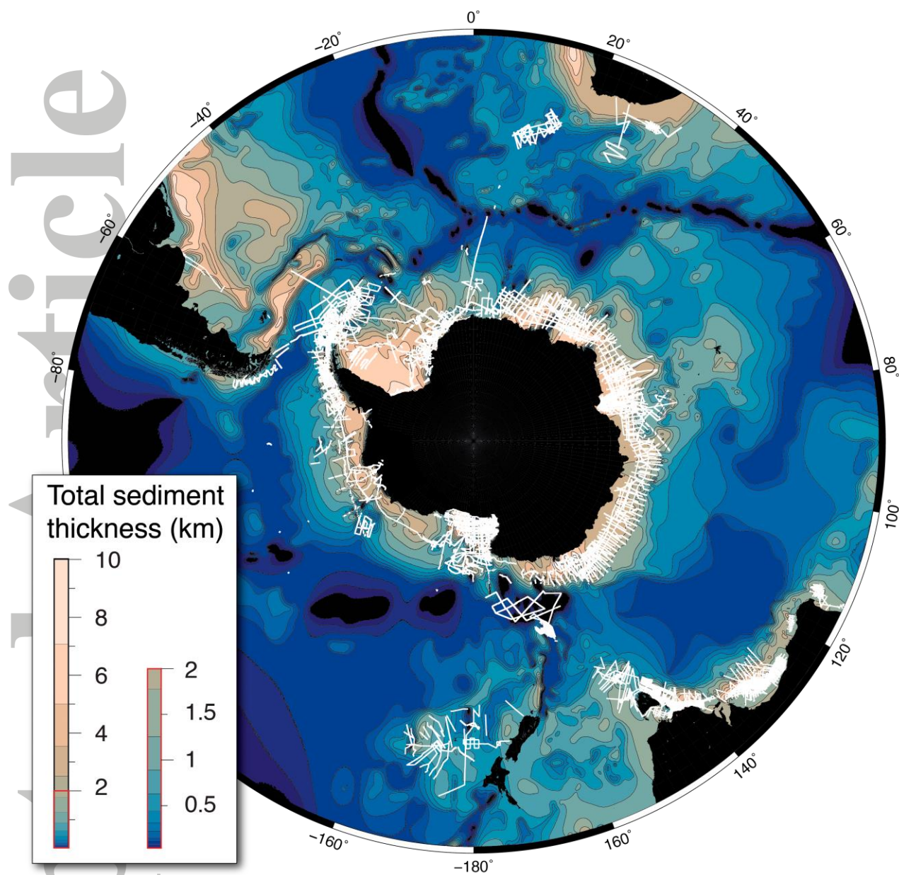
Figure 4: Southern Ocean total sediment thickness with locations of seismic lines (white lines).
