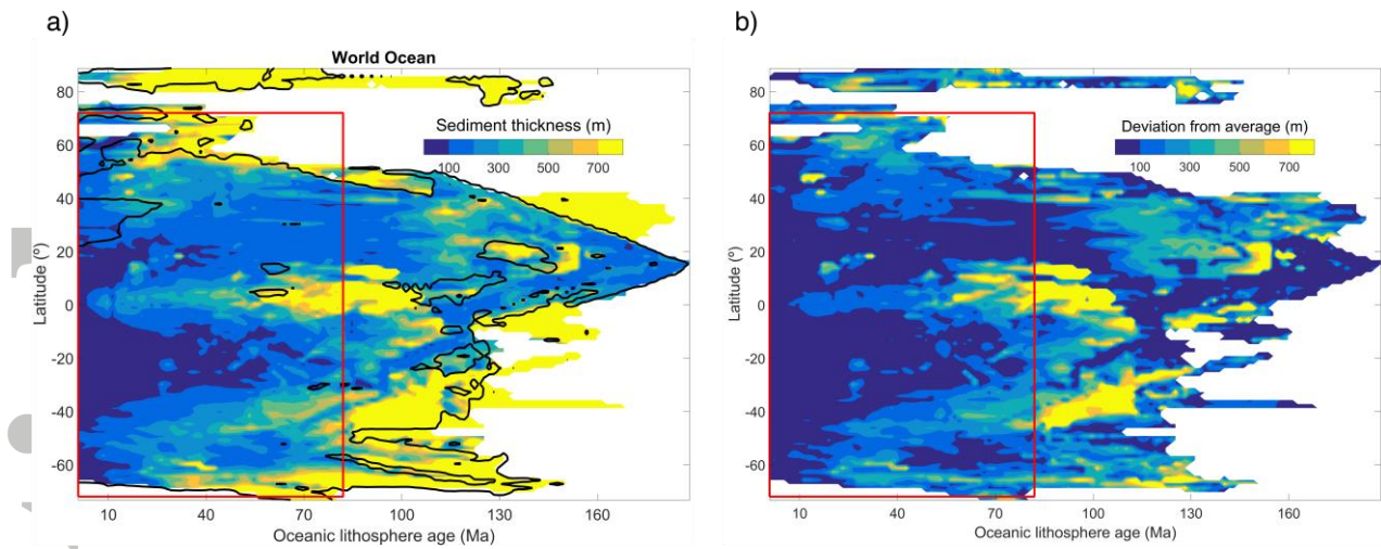
Figure 9: Values of average sediment thickness (a) and standard deviation (STD, b) for considered sediment data (see text for details of excluded data) distributed over bins 1.5 My by 1.5° of latitude. Black line in (a) cuts out areas with few data (less than 130 data in each bin). Red rectangle outlines area considered in more detail.
