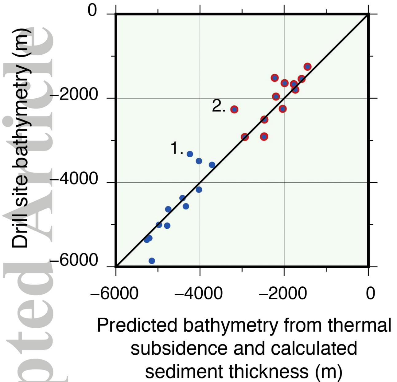
Figure 13: This is the same as in Fig. 12g updated for residual bathymetry of LIPs. See text for a more detailed explanation, and supplementary material for the outliers marked 1 and 2.
