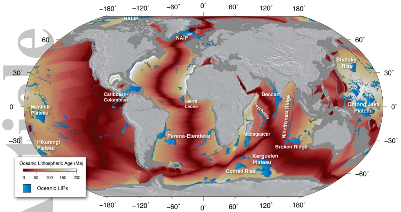
Figure 7: Age of the oceanic lithosphere (see text for details). Oceanic Large Igneous Provinces (LIPs) from Torsvik & Cocks (2016) are colored in light blue. NAIP = North Atlantic Igneous Province, HALIP = High Arctic Large Igneous Province.
