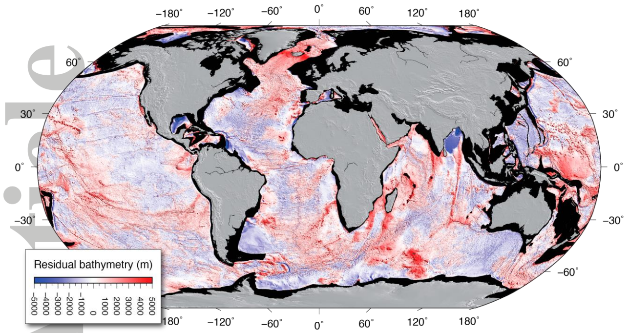
Figure 8: Global residual bathymetry of the oceanic lithosphere.
