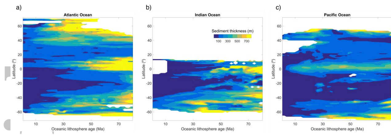
Figure 10: Distribution of average sediment thickness for Atlantic (a), Indian (b) and Pacific (c) oceans. The data analysis is restricted to max. 82 Ma age of the oceanic lithosphere and up to 72° of latitude (north and south).
