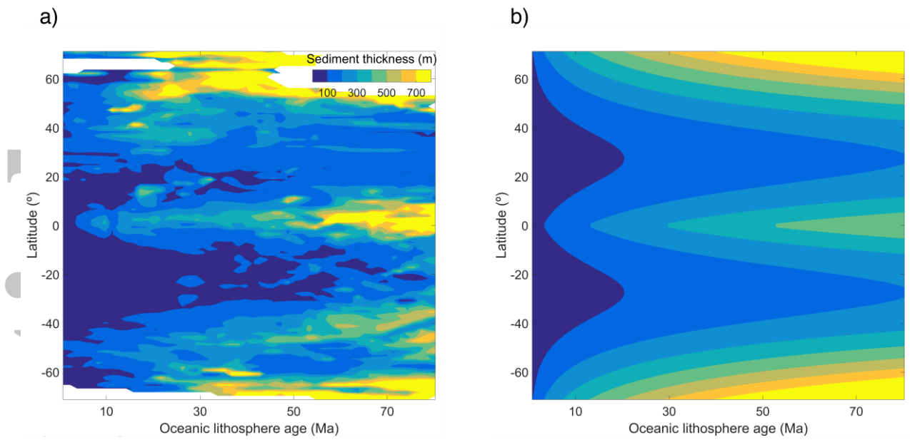
Figure 11: (a) Distribution of average sediment thickness in world's ocean for the parameter space restricted by the red rectangle in Fig. 9. (b) Analytical approximation of the average sediment thickness described by eq. 2.
