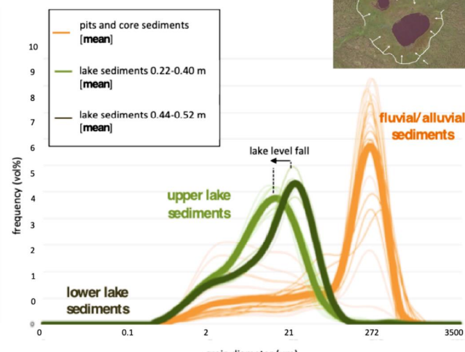
Frequency of mean grain sizes of all section sediments and lake sediments. Note: Lower lake sediments are coarser than upper lake sediments. Uppermost layer (0.00-0.22 m) is organic detritus only.
