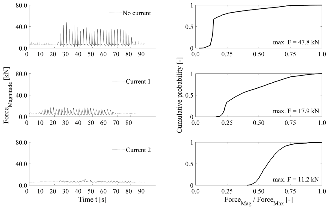
Fig. 6. Force evaluation based on the single configuration of the model for all three current velocities and a wave height of 4.0 m and wave period of 10 s (in prototype scale) propagating from 90°. Empirical cumulative distribution function for each case on the right.
