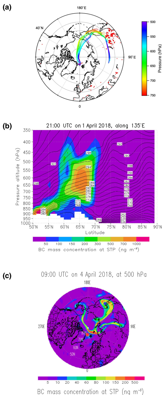
Figure 7. (a) Eight-day backward trajectories of air with enhanced BC mass concentrations ( M_{\text{BC}} ) observed on 2, 3, and 4 April 2018 (the data points shown in red in Fig. 2a). Red points are MODIS-derived hot spots observed during 25–27 March, 8 d before the aircraft observations of the enhanced M_{\text{BC}} . (b) Model-calculated latitude–pressure–altitude cross-section of M_{\text{BC}} along the 135° E line (color) and potential temperature (contours) at 21:00 UTC on 1 April 2018 (MRI-ESM2 model). M_{\text{BC}} values originating from BB are shown. (c) Horizontal distribution of M_{\text{BC}} (BB origin) at 500 hPa level at 09:00 UTC on 4 April 2018 when the enhanced M_{\text{BC}} data were observed (MRI-ESM2 model). The red circle denotes the aircraft location when the enhanced M_{\text{BC}} data were observed.
