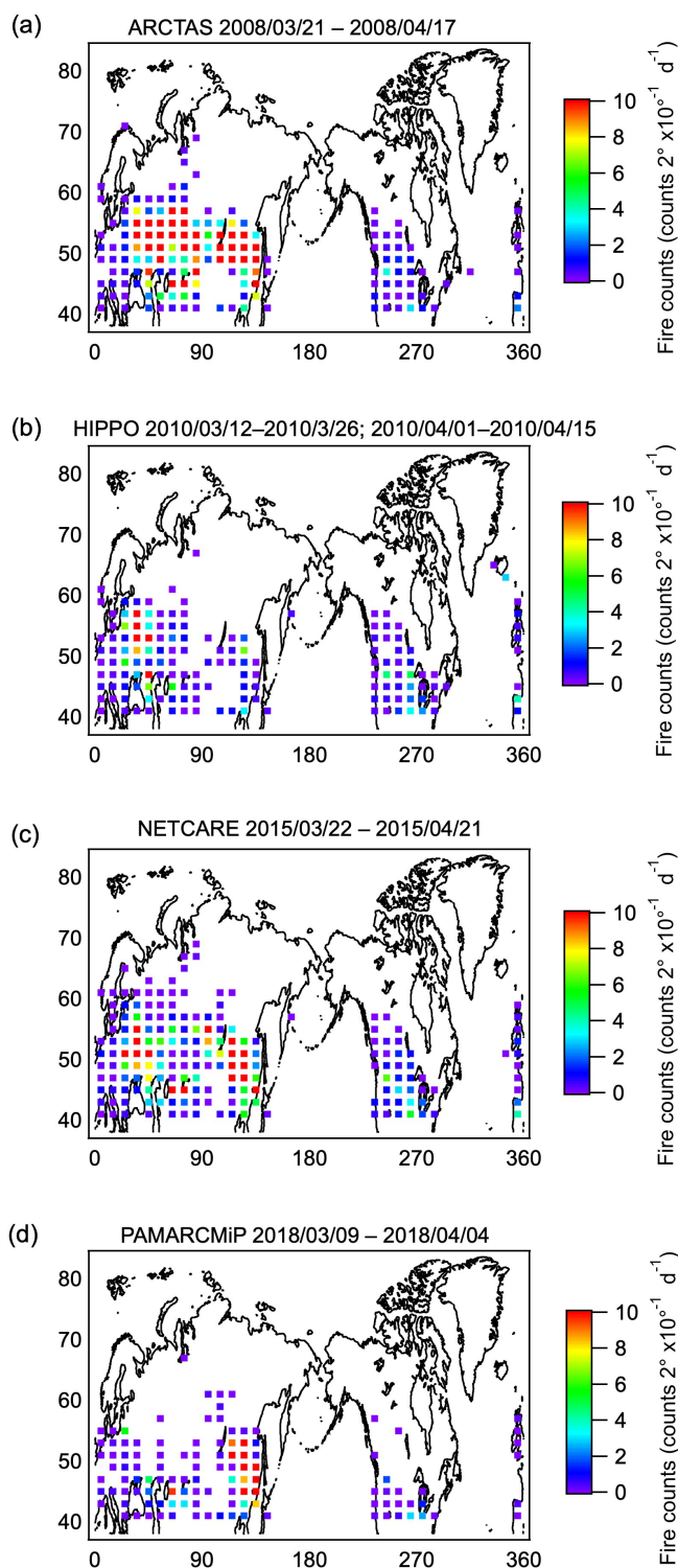
Figure 4. Map of MODIS-derived fire counts. Averaged values are shown for the time period between 14 d before the first day of an aircraft-based experiment and the last day of the experiment.
