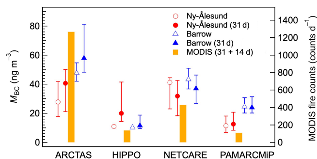
Figure 6. BC mass concentrations ( M_{\text{BC}} ) obtained by ground-based measurements at Ny-Ålesund, Svalbard (red), and Barrow, Alaska (blue). Median values of daily averages and 25%–75% ranges are shown for the time periods of the individual aircraft experiments (open circles and triangles) and the 31 d period for which the median date was chosen to be the median date of the experiment (closed circles and triangles). Corresponding averaged fire counts (31 + 14 d) at latitudes north of 50^\circ\text{N} are also shown (vertical bars). Because the daily averaged M_{\text{BC}} was obtained only on 1 d at Barrow for the HIPPO experiment period (2 d), the 25%–75% range is not shown.
