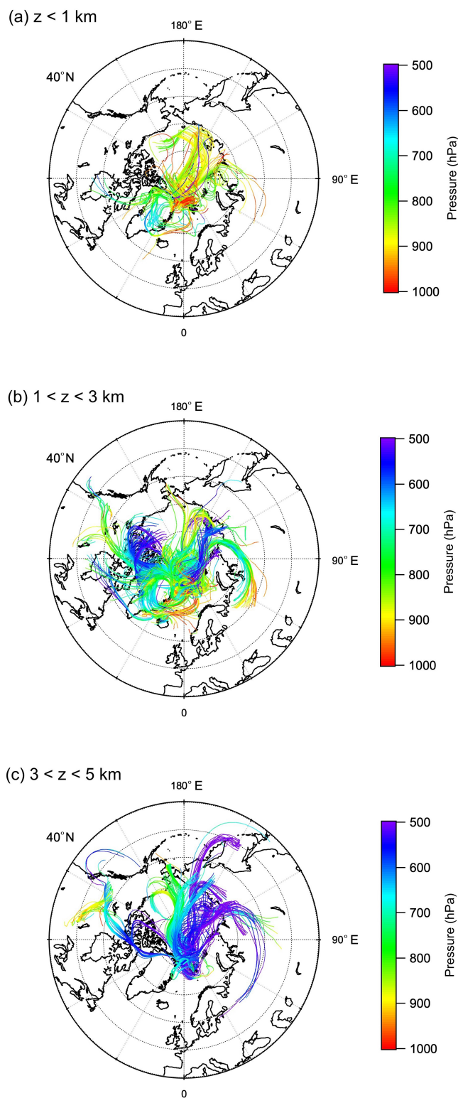
Figure B1. Six-day kinematic back trajectories of air parcels measured aboard the aircraft. Color scales denote the pressure altitude of air. (a) Trajectories starting from altitudes z < 1 km. (b) Same as (a) but for 1 < z < 3 km. (c) Same as (a) but for 3 < z < 5 km.
