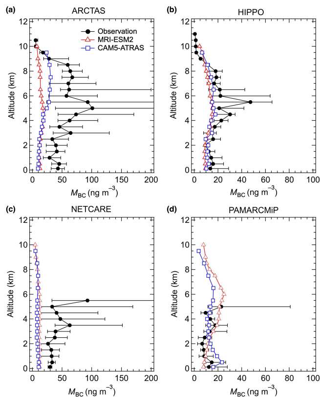
Figure D1. Vertical profiles of median BC mass concentration ( M_{\text{BC}} ) values observed during the aircraft-based experiments made over the Arctic ( >66.5^\circ\text{N} ) in spring. Bars indicate 25%–75% ranges. Model-calculated vertical M_{\text{BC}} profiles are derived by calculating area-weighted averages within the latitudes and longitudes and the time periods of the individual aircraft-based experiments.
