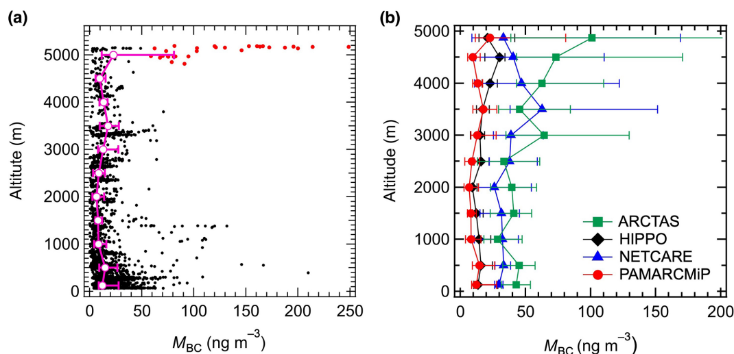
Figure 2. (a) Vertical profile of the BC mass concentration ( M_{BC} ) observed during the PAMARCMiP aircraft-based field experiment. Closed circles denote 1 min data. Median values and 25 %–75 % ranges are also shown. Data points shown in red (enhanced M_{BC} data points) were likely influenced by biomass burning emissions and are discussed in Sect. 5. (b) Vertical profiles of median M_{BC} values observed during the aircraft-based experiments made over the Arctic ( >66.5^{\circ} N) in spring (Table 3).
