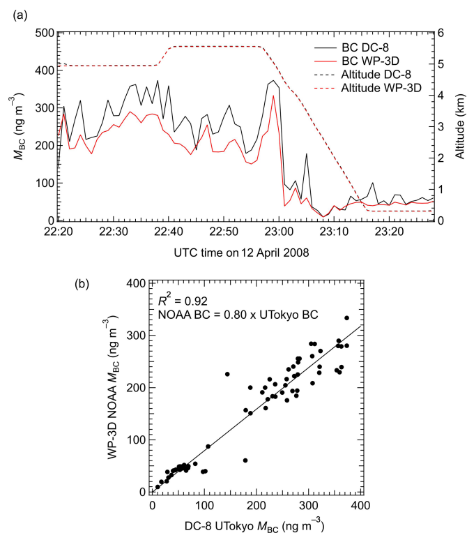
Figure A1. Comparison between M_{BC} measurements made with The University of Tokyo SP2 during ARCTAS aboard the NASA DC-8 (black lines; Sahu et al., 2012) and NOAA SP2 measurements aboard the NOAA WP-3D (red lines, NOAA-ARCPAC experiment; Spackman et al., 2010). (a) Time series of 1 min data of M_{BC} values (solid lines) and aircraft altitudes (dashed lines). (b) Scatterplot between these M_{BC} values. The solid line is the least-squares fitted line forced through (0, 0).
