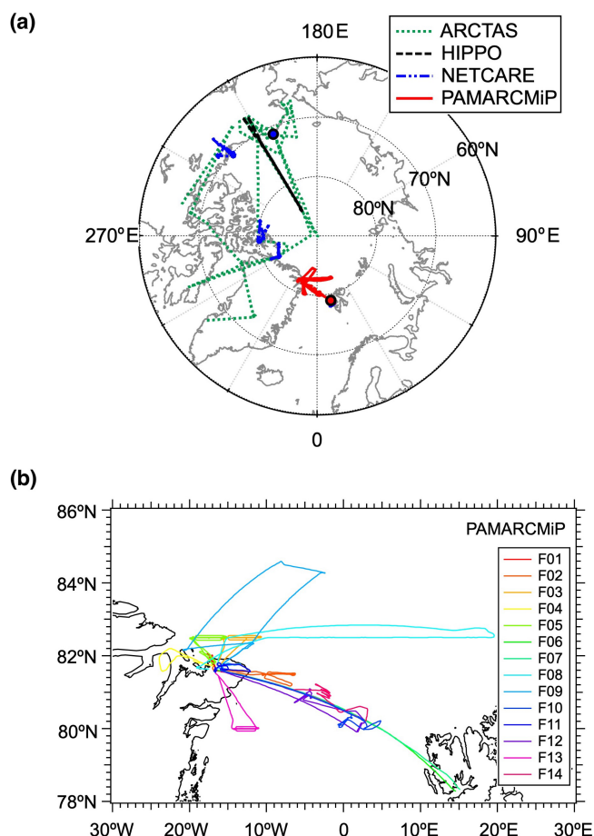
Figure 1. (a) Map of the flight tracks of the PAMARCMiP aircraft-based field experiment and the other three experiments made over the Arctic in spring. In this study, only data obtained at latitudes north of 66.5^{\circ} N were used and only the flight tracks for them are shown. The locations of the high Arctic sites Ny-Ålesund in Svalbard ( 78.9^{\circ} N, 11.9^{\circ} E) and Barrow in Alaska ( 71.3^{\circ} N, 156.6^{\circ} W) are indicated by the red and blue circles, respectively. (b) Map of the details of the flight tracks of the PAMARCMiP experiment.
