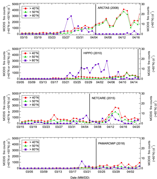
Figure C1. Time series of the daily averaged number of fire counts (counts \text{d}^{-1} ) detected by the MODIS satellite. Vertical bars indicate the start dates of the individual aircraft-based experiments.
