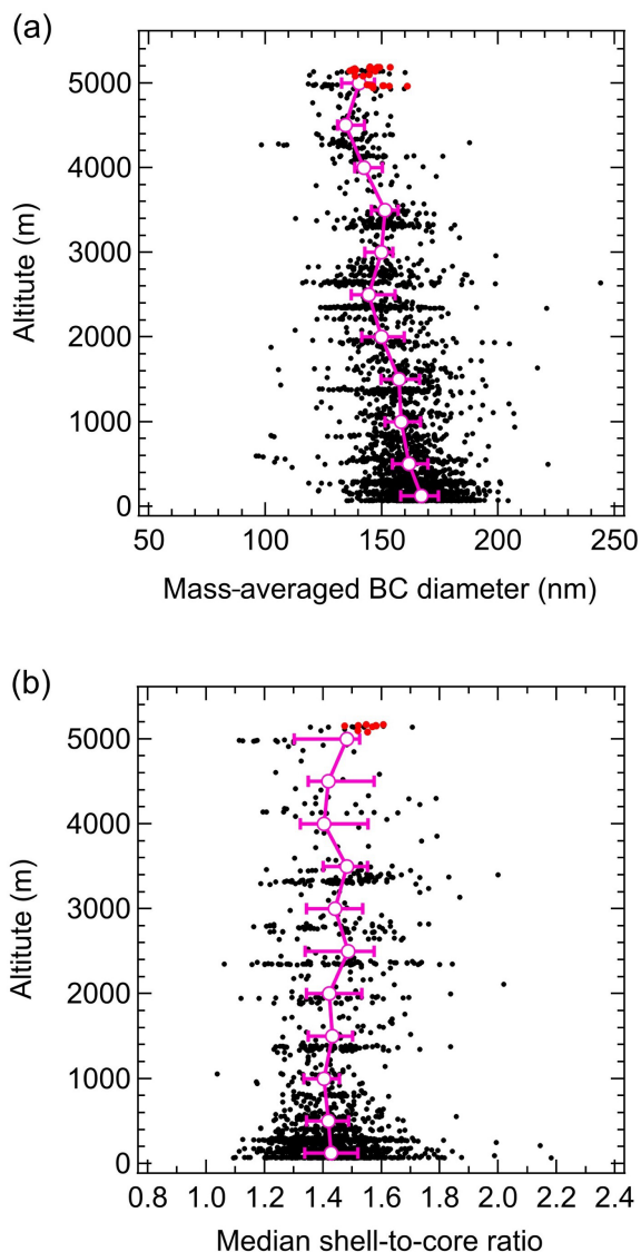
Figure 8. (a) Vertical profile of mass-averaged diameters of BC ( D_{BC} ). Closed circles denote 1 min data that were calculated from 1 min BC mass concentrations ( M_{BC} ) and BC number concentrations using Eq. (1). Median values and 25%–75% ranges are also shown. Data points shown in red (the enhanced M_{BC} data points shown in red in Fig. 2a) were likely influenced by biomass burning emissions. Panel (b) is the same as (a) but for the median shell-to-core diameter ratios for particles with a mass equivalent BC diameter (core diameter) of 180–192 nm.
