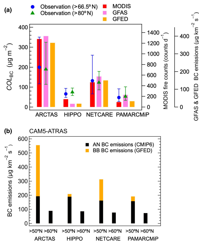
Figure 3. (a) Column amounts of BC mass concentration at altitudes between 0 and 5 km ( COL_{BC} ) at latitudes north of 66.5^\circ\text{N} (blue circles) and 80^\circ\text{N} (green triangles). MODIS-derived fire counts and biomass burning BC emissions compiled in GFAS and GFED datasets are also shown (vertical bars). The fire counts and BC emissions are those at latitudes north of 50^\circ\text{N} for the time period between 14 d before the first day of an aircraft experiment and the last day of the experiment. (b) BC emissions used for the CAM5-ATRAS model simulations. Anthropogenic (AN, CMIP6) and biomass burning (BB, GFED) emissions are shown by black and orange colors, respectively. Values at latitudes north of 50 and 60^\circ\text{N} are shown for the time period between 14 d before the first day of an aircraft experiment and the last day of the experiment. The BB emissions for >50^\circ\text{N} are the same as those shown in Fig. 3a. BC emissions used for the MRI-ESM2 model simulations (MAC-City and GFAS) are generally similar to those shown in this figure, although AN emissions for >60^\circ\text{N} are generally smaller.
