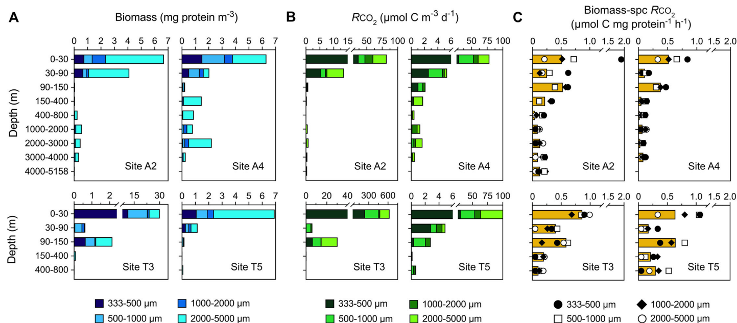
Fig 3. (A) Protein content and (B) respiration rates of each zooplankton size class across depth strata in those stations where plankton nets were deployed. (C) Protein-specific respiration rates, with yellow bars standing for the mean specific rates and symbols representing the individual rates of the corresponding size fractions. Note the changes in x-axis scales for Site T3.
