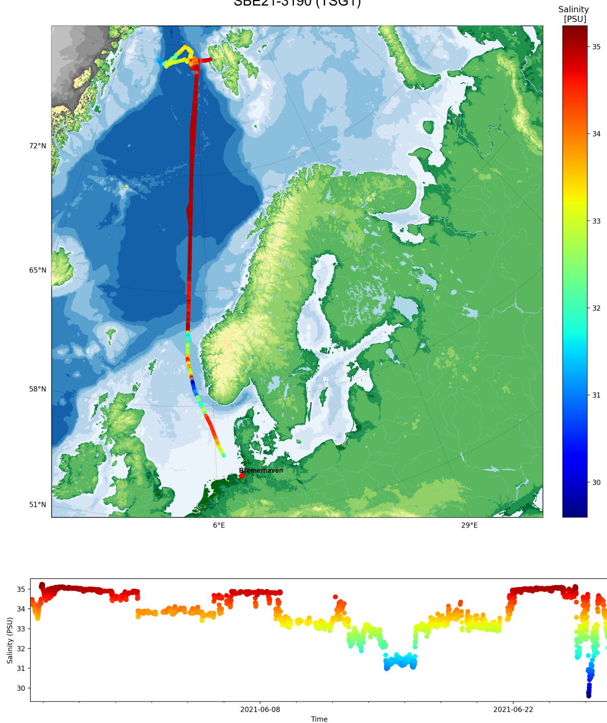
Salinity data from Polarstern cruise PS126 SBE21-3190 (TSG1)
