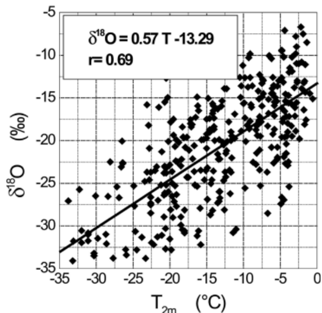
Fig. 4. Correlation of \delta^{18}\text{O} values of fresh-snow samples and 2 m air temperature at Neumayer station, 1981–2000.
